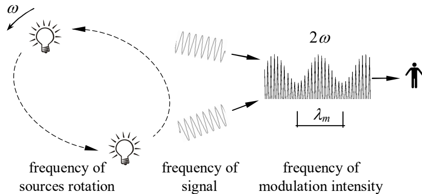
Fig. 15. Frequency of light intensity modulation is something else than the frequency of light signal.
