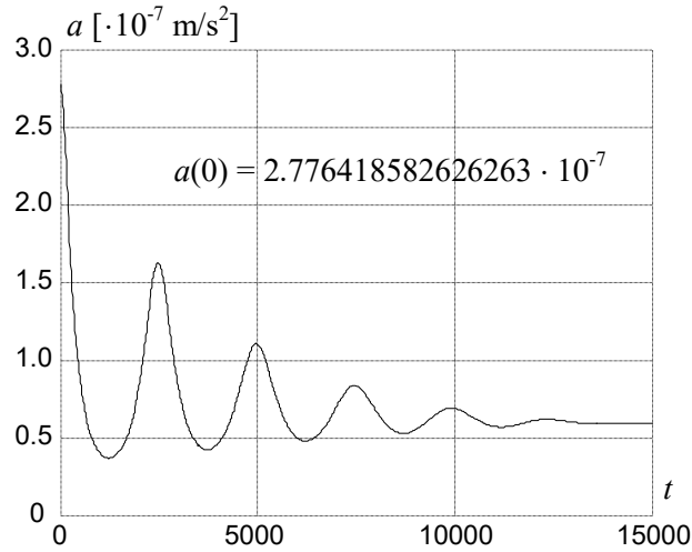
Fig. 3. The gravitational field intensity for D = 1.5 m, r(0) = 1 m, m_1 = m_2 = 1\,000 kg, T = 5\,000 .
