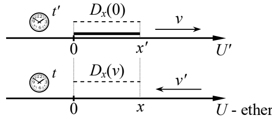
Fig. 7. Inertial system moves in relation to the ether with speed v , while the ether moves in relation to the inertial system with speed v' ( v \cdot v' \leq 0 ).
